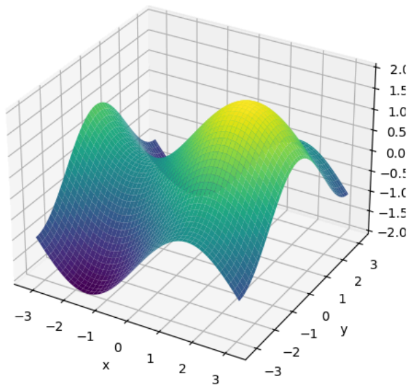
Original Function: \sin(x) + \cos(y)
